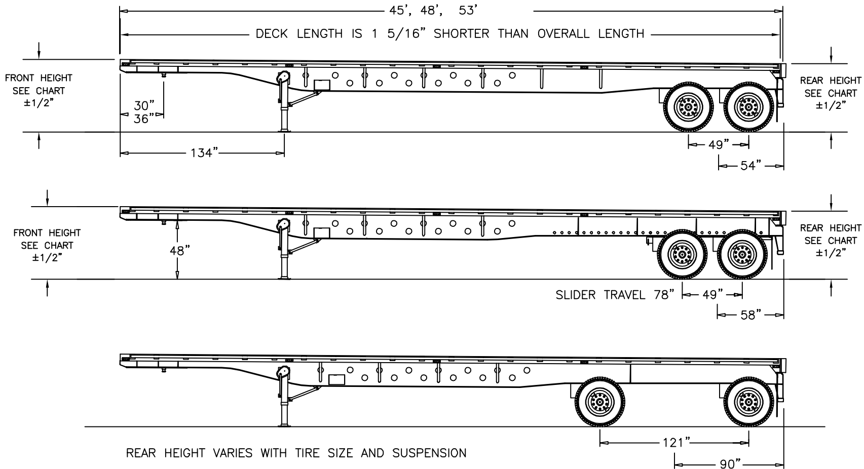
REAR HEIGHT VARIES WITH TIRE DIAMETER AND SUSPENSION SETTING
